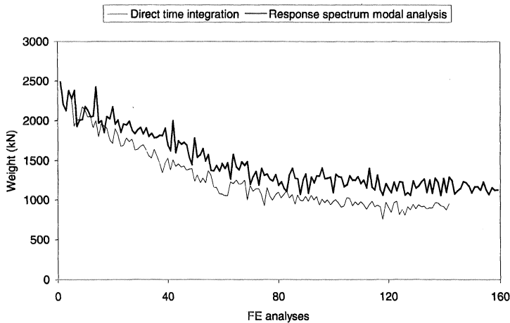
Fig. 5. Convergence histories of the optimization procedure.
