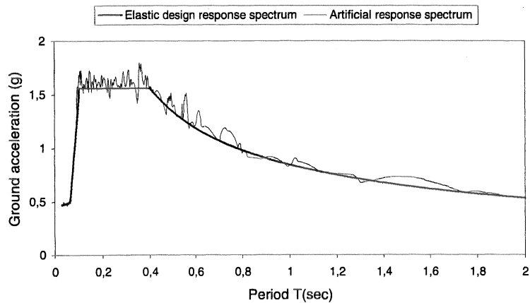
Fig. 1. Elastic design response spectrum of the region and response spectrum of the first artificial accelerogram ( \xi = 2.5\% ).
