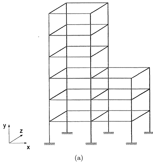
Fig. 4. (a) Six storey space frame; (b) element groups.
