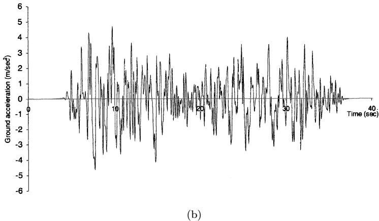
Fig. 2. The five artificial accelerograms.
